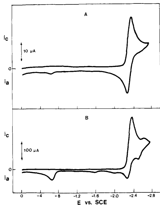
Figure 1. Cyclic voltammograms in 0.2 M TBAP-DMF at a scan rate of 0.1 V s -1 (A) 5.2 × 10 -4 M 4-cyanodiphenyl ether, (B) 5.4 × 10 -3 M 4-cyanodiphenyl ether. The planar platinum electrode area was 0.20 cm 2 .
