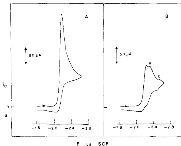
Figure 6. Cyclic voltammograms of 4.7 \times 10^{-2} M 2-cyanodiphenyl ether in 0.2 M TBAP-DMF: (A) before electrolysis and (B) after electrolysis at E_{app} = -2.25 V with the addition of 1.2 F mol -1 . The scan rate was 0.1 V s -1 on a platinum-bead electrode.
