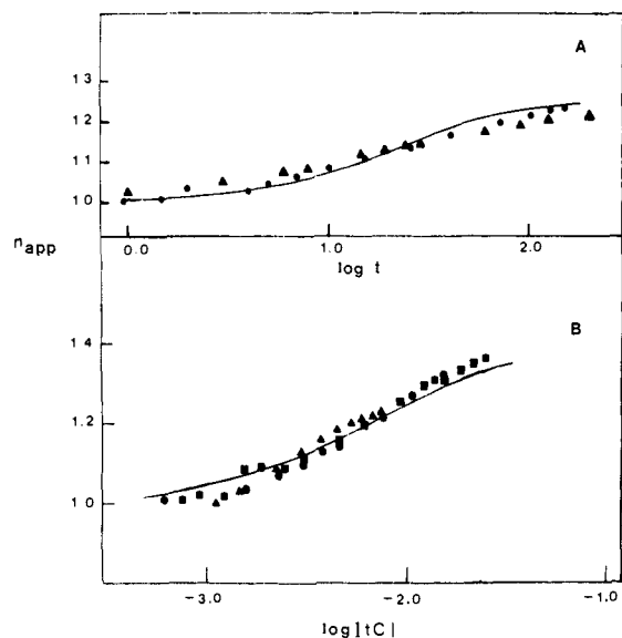
Figure 4. Single-potential-step chronoamperometric data for the change in electron stoichiometry or product formation in the reduction of 4-cyanodiphenyl ether in 0.2 M TBAP-DMF: (A) E_{app} = -2.43 V on a planar, shielded platinum electrode (0.28 cm 2 ); (B) E_{app} = -2.75 V on a planar platinum electrode (0.20 cm 2 ). The solid curves were obtained by computer simulation 17,20 of: (A) eq 5–7 with a first-order rate constant ( k_1 ) of 3.8 \times 10^{-2} s -1 ; (B) eq 8–12 with a second-order rate constant ( k_2 ) of 9.6 \times 10^1 M -1 s -1 and K_{eq} = 10^{-4} . 22 The experimental points are for concentrations of 4-cyanodiphenyl ether: (A) (●) 3.74 \times 10^{-3} M, (▲) 1.99 \times 10^{-2} M; (B) (▲) 7.4 \times 10^{-3} M, (●) 1.53 \times 10^{-2} M, (■) 3.06 \times 10^{-2} M.
