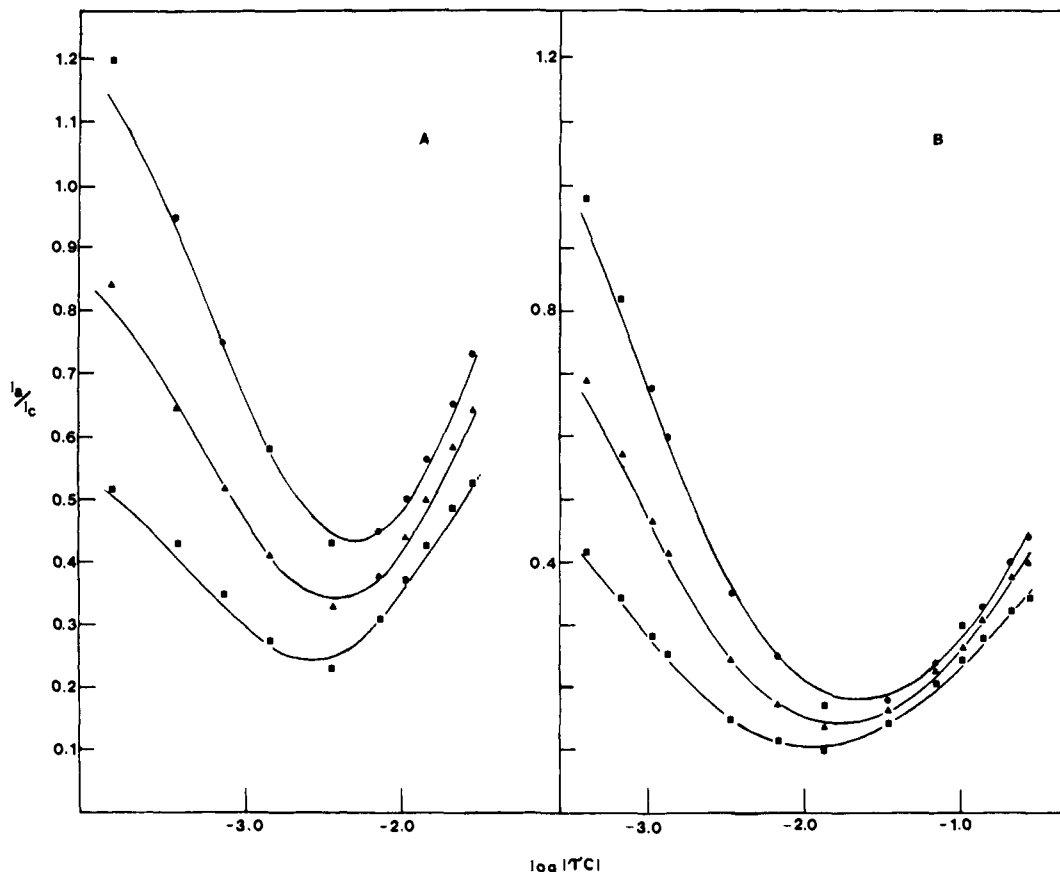
Figure 7. Double-potential-step chronoamperometric data for the disappearance of the 2-cyanodiphenyl ether radical anion in 0.2 M TBAP-DMF. The solid curves were obtained by computer simulation 17 of the processes described by eq 14 and 15 with (A) k_f = 1.2 \times 10^3 \text{ M}^{-1} \text{ s}^{-1} and k_b = 1.0 \times 10^{-1} \text{ s}^{-1} at 1.44 \times 10^{-3} \text{ M } 2 and (B) k_f = 1.1 \times 10^3 \text{ M}^{-1} \text{ s}^{-1} and k_b = 9.2 \times 10^{-2} \text{ s}^{-1} at 1.35 \times 10^{-2} \text{ M } 2 . The ratios of t_a/\tau were: (●) 0.2; (▲) 0.3; (■) 0.5, where \tau = cathodic electrolysis time and t_a = anodic electrolysis time.
